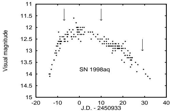
Fig. 2. Visual light curve of the SN1998aq based on the VSNET data bank. Arrows indicate the epochs of spectroscopic observations.
